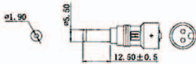
3. \varnothing 1.90 \times 5.50 \times 12.5 \pm 0.5 mm "I" type
